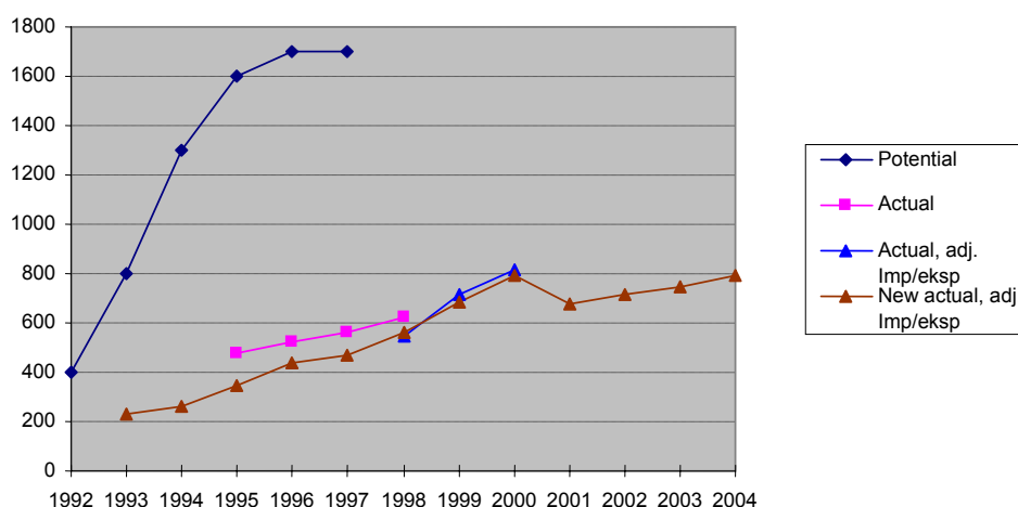
Figure 1.4 Trends in GWP-weighted potential, actual and adjusted actual emissions 1992-2004, 1000 tonnes CO 2 equivalents.
