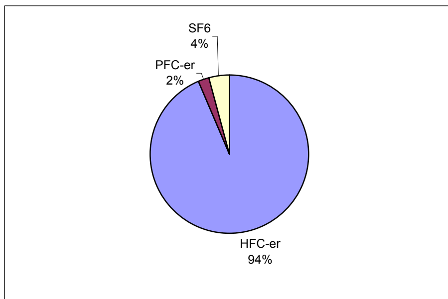
Figure 1.3 The relative distribution of the GWP contribution from HFCs, PFCs, and SF 6 , 2004.
