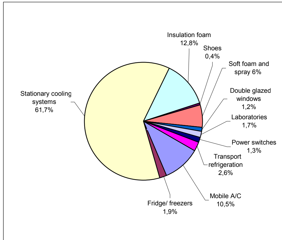
Figure 1.2 The relative distribution in 2004 of GWP contribution, analysed by source
