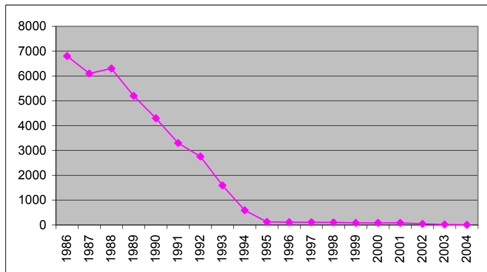
Figure 1.1 The development of ODP-weighted consumption 1986-2004, tonnes.
