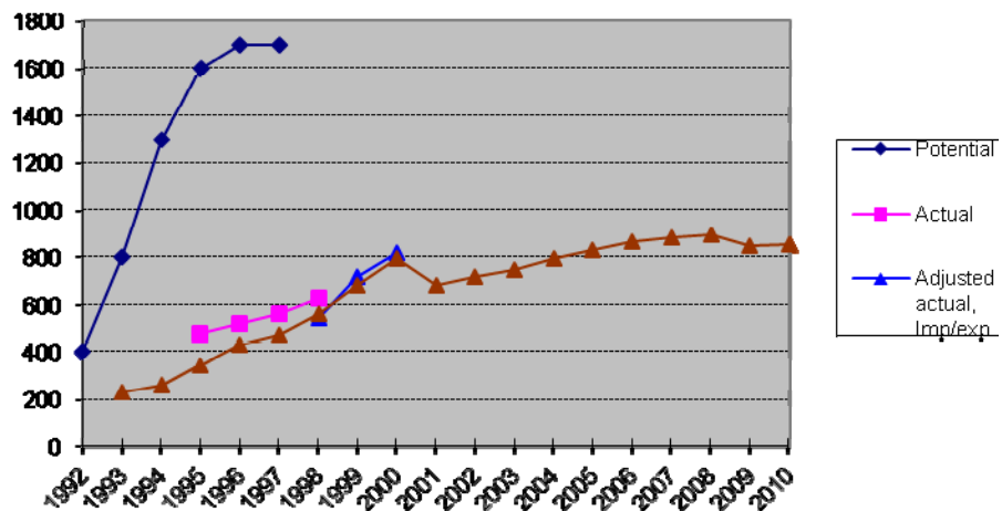
Figure 1.3 Trends in GWP-weighted potential, actual and adjusted actual emissions 1992-2010, 1,000 tonnes CO 2 equivalents.
