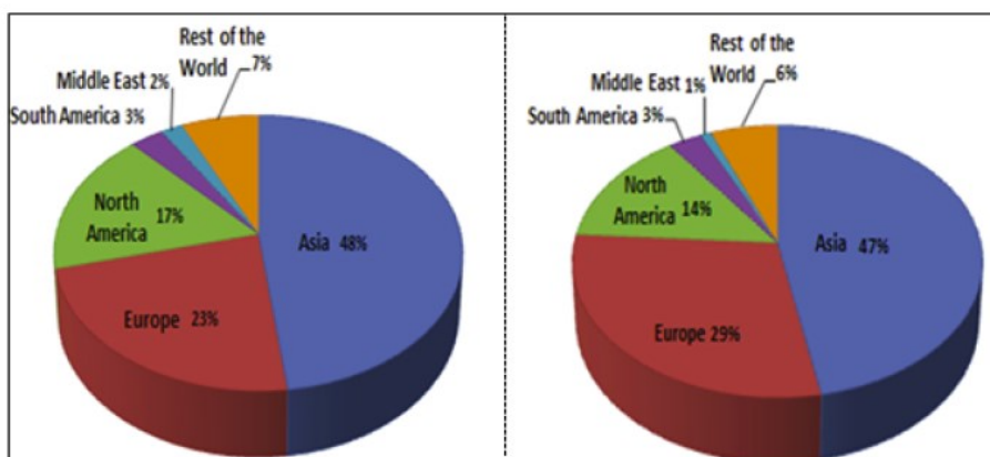
FIGURE 3-1 GLOBAL FORMALDEHYDE PRODUCTION (LEFT FIGURE) AND CONSUMPTION (RIGHT FIGURE) BY MAJOR REGIONS IN 2008 (FIGURE TAKEN FROM ICF, 2013).
