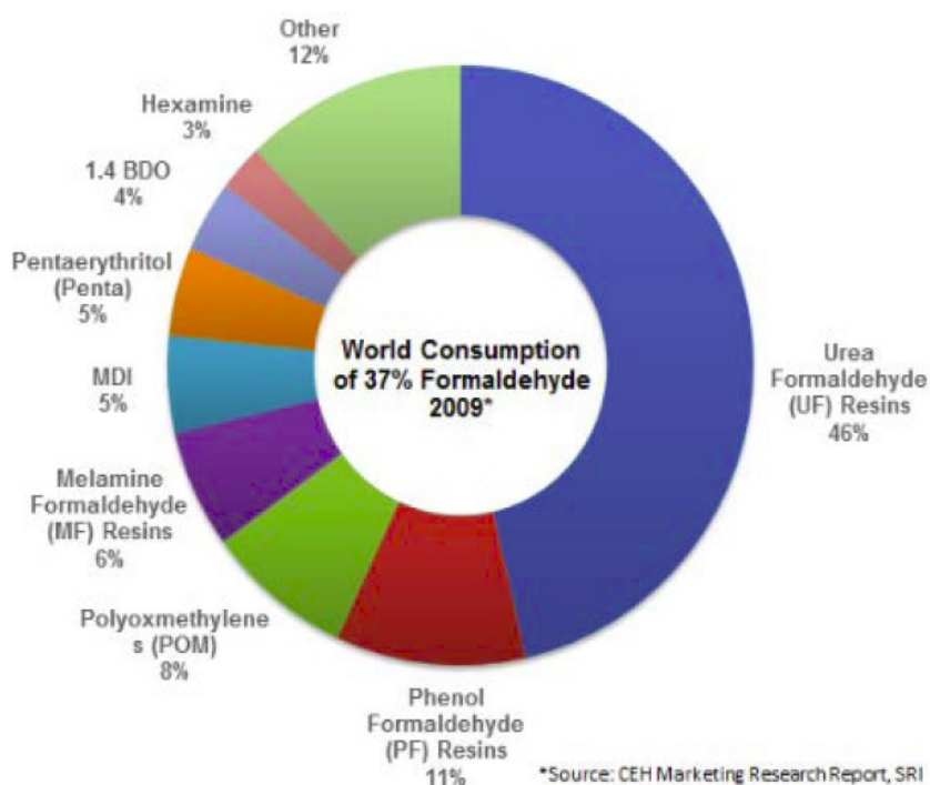
FIGURE 3-2 WORLD CONSUMPTION OF FORMALDEHYDE FOR USE IN THE PRODUCTION OF FORMALDEHYDE RESINS AND SPECIALTY CHEMICALS (FIGURE TAKEN FROM ICF, 2013)
