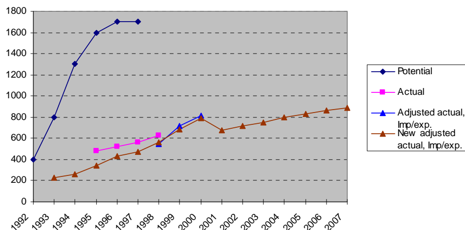
Figure 1.3 Trends in GWP-weighted potential, actual and adjusted actual emissions 1992-2007, 1,000 tonnes CO 2 equivalents.
