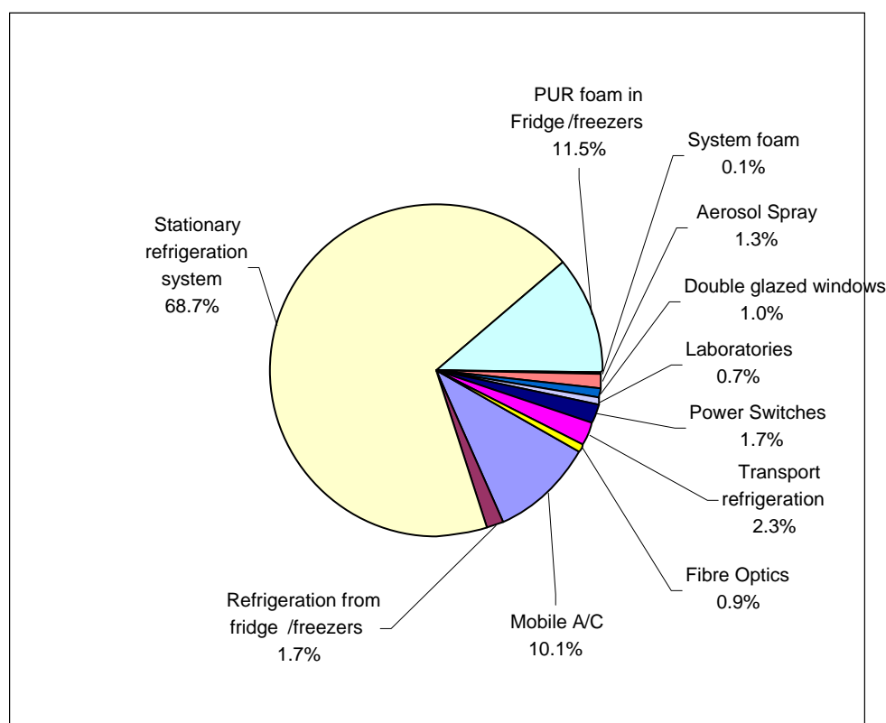
Figure 1.1 The relative distribution of GWP emissions, analysed by application area, 2007
