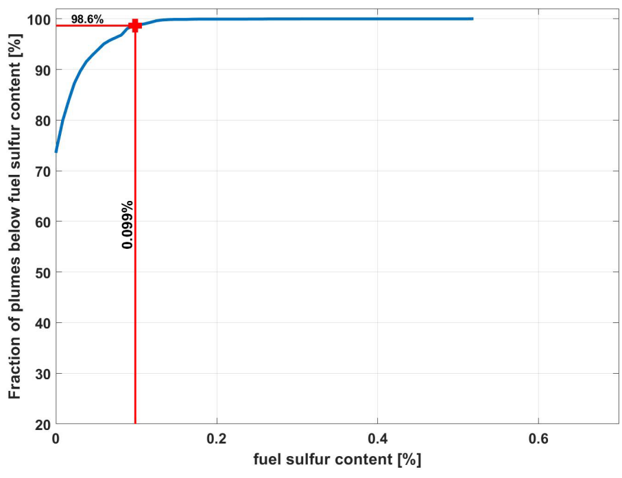
FIGURE 11. The fraction of ships that were measured below a certain FSC level at the Great Belt Bridge for the period December 2018 to November 2019. In addition, the biased corrected compliance limit threshold is shown.
