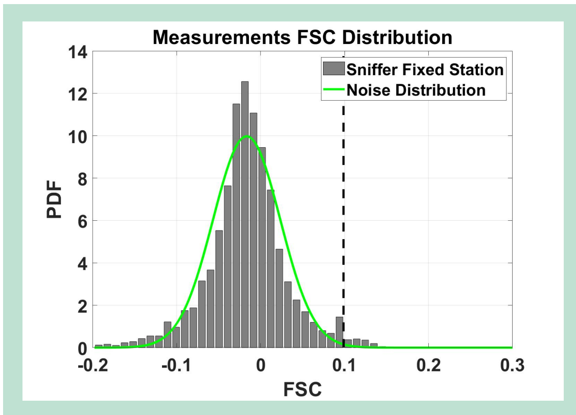
FIGURE 9. Statistical distribution (probability density function) of the measured FSC, corresponding to individual ships measured with sniffer at the Great Belt Bridge. The data covers the period December 2018 to November 2019. The green curve corresponds to the random noise distribution (precision) of the measurements obtained from multiple measurements of single ships. The dotted line is the estimated non-compliance limit for which the instrument errors (precision and bias) have been accounted for. The measured data set has a median and average FSC values of -0.016% and -0.0159 %, respectively. The standard deviation is 0.0473 % and the 75 th and 90 th percentiles are 0.007% and 0.037 % in FSC units, respectively.
