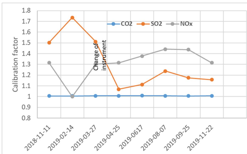
FIGURE 6. The calibration factors obtained during 2019 through measurements of gas standards from Air liquide.
