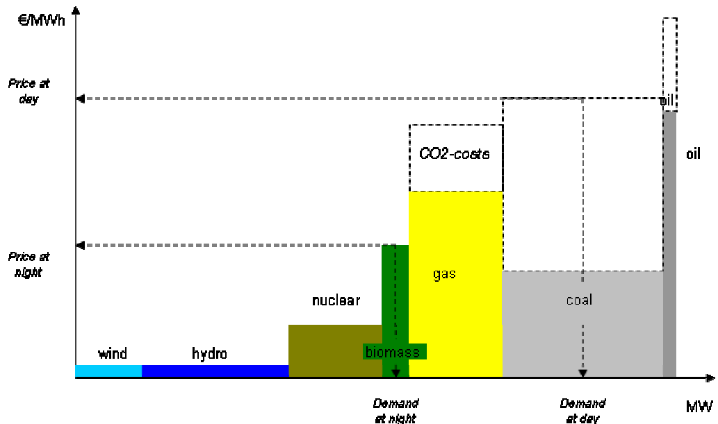
Figure 11: Supply and demand in the electricity spot-market, including CO 2 .
