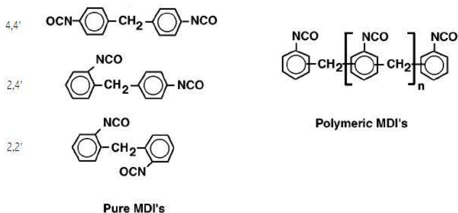
FIGURE 2 MDI ISOMERS
